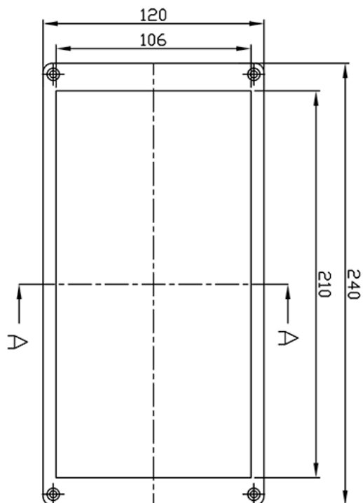
VIEW OF LID
