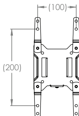
MOUNTING PROFILE
