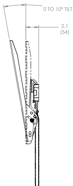
MOUNTING PROFILE
