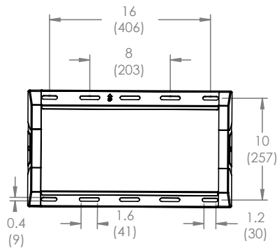
WALL MOUNT BRACKET
