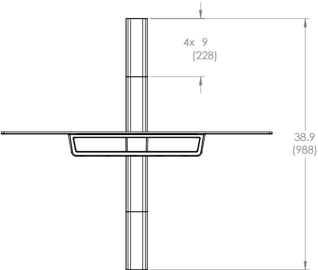
SHELF WITH CABLE MANAGEMENT
