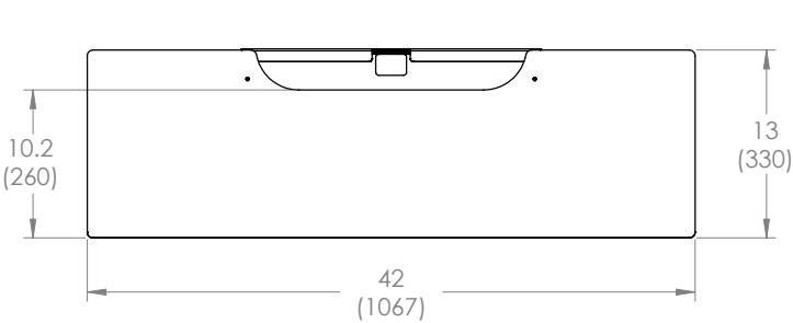
GLASS DIMENSIONS
