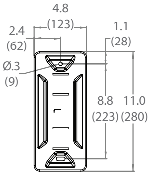
WALL MOUNTING
