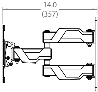
MAXIMUM EXTENSION
