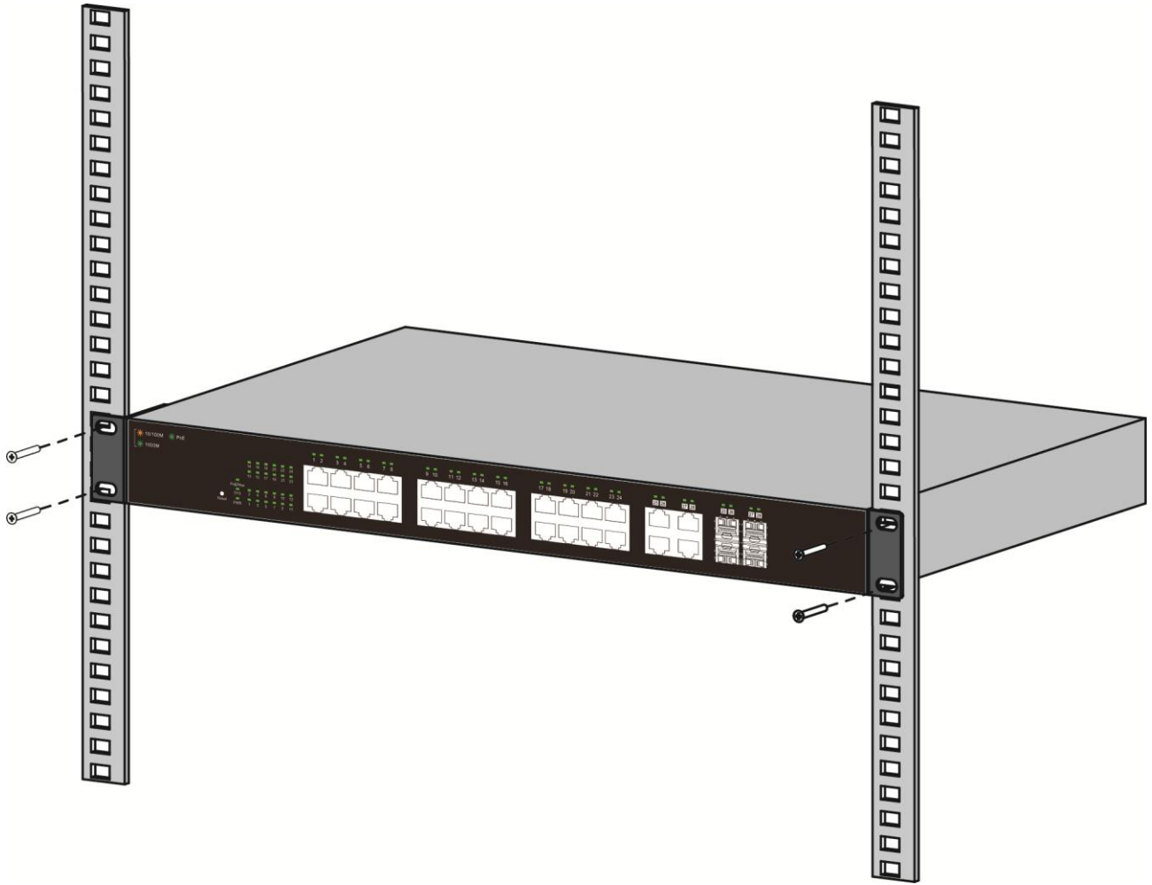
Figure 6 - Rack Installation
