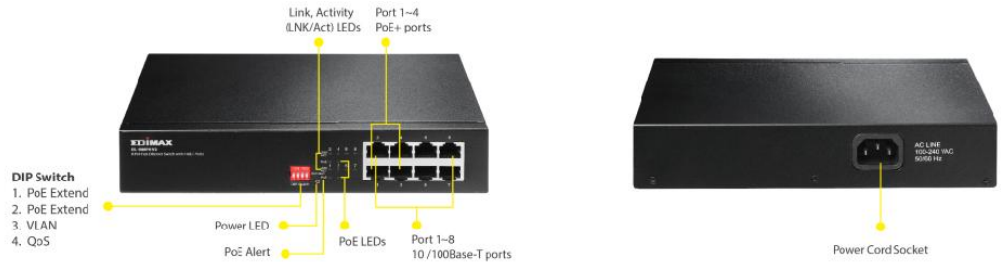
Front Panel
