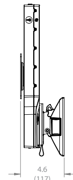
SIDE VIEW (NESTED)
