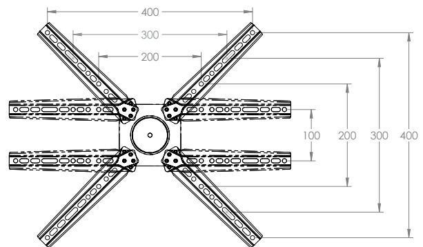
VESA PLATE WITH ADAPTERS (mm)
