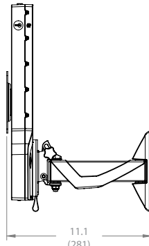
SIDE VIEW (EXTENDED)
