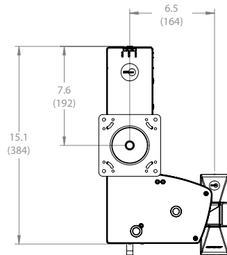
FRONT VIEW (NESTED)
