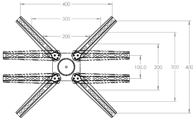
VESA PLATE WITH ADAPTERS (mm)
