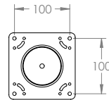
VESA PLATE (mm)
